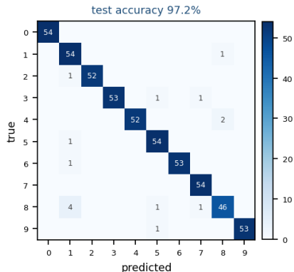
Confusion matrix, linear classifier on digits
